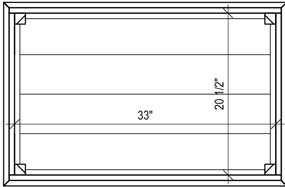
BOX TOP VIEW
