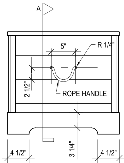
BOX FRONT VIEW
