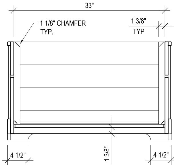
BOX SECTION 'A'
